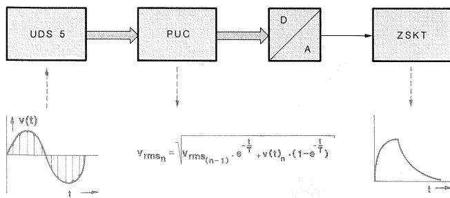
FIG 2 Determining rms value of very low-frequency signals in point-by-point measurements using high-speed Digital Multimeter UDS 5. Time response of rms value calculated by controller may be recorded via D/A converter (here transient response and decay after switching signal on and off).
