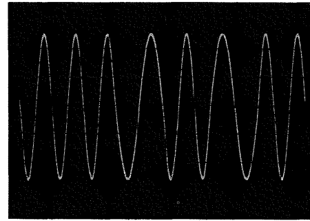
FIG 4 Section of NMT telegram generated by SCUD showing precise frequency change during zero-crossing (logic 1 = 1 period 1200 Hz, logic 0 = 3/2 periods 1800 Hz).
