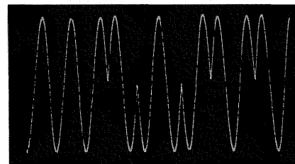
FIG 9 Section of PSK data telegram as example of exact generation by SCUD.
