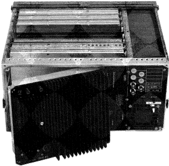
FIG 14 Easy service and maintenance design of CMT. Few and large plug-in cards are connected via common motherboard and replaceable without readjustment. Power supply can be removed after loosening few screws and can even be loaded when dismantled for service purposes.
