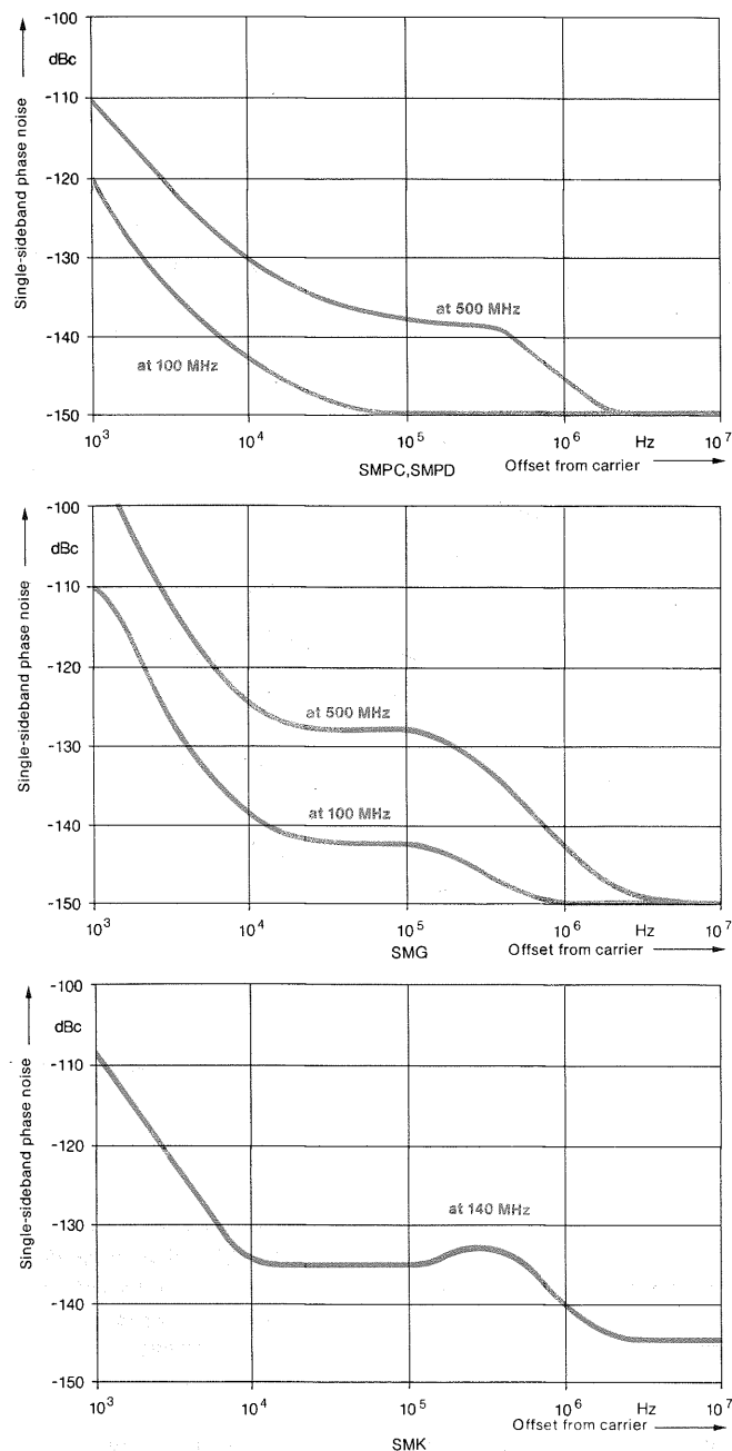
FIG 2 SSB phase noise with 1 Hz bandwidth as function of offset from carrier.
