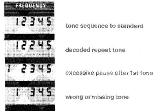
FIG 15 Display of decoded selective-call sequences on frequency display of SMFP 2/SMFS 2.
