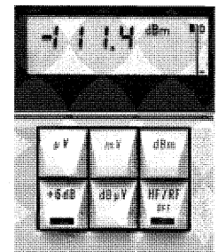
FIG 12 SMFP 2 and SMFS 2 output-level display combined with read-out of electronic, fine level variation with keys for entry and conversion of physical units.
